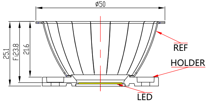
OPTICAL ASSEMBLY DIAGRAM
